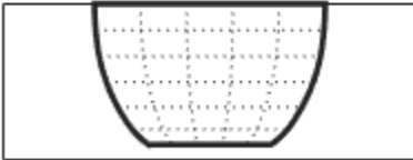
Lat [-90 0], Lon [-180 -30]
