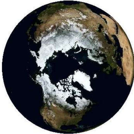
Blue Marble
